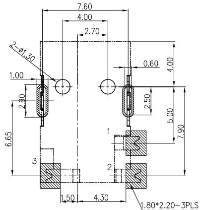
RECOMMENDED PADS LAYOUT <TOP VIEW>
