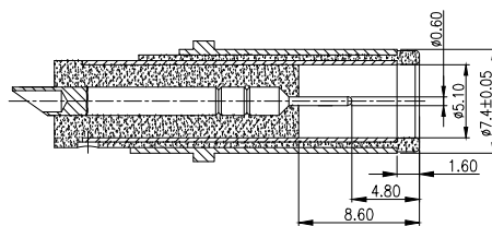
MATING PLUG: OD \phi 7.4 ; ID \phi 0.6 Tolerance: \pm 0.05
