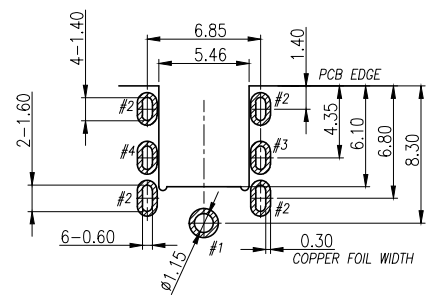
RECOMMEND P.C.B LAYOUT (TOLERANCES:±0.05)
