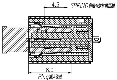
<4.>Plug full Mating狀態
