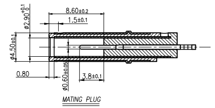
PLUG 规格 45P06CV230-1A00-01
