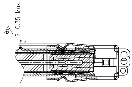
SECTION A-A PLUG IN
