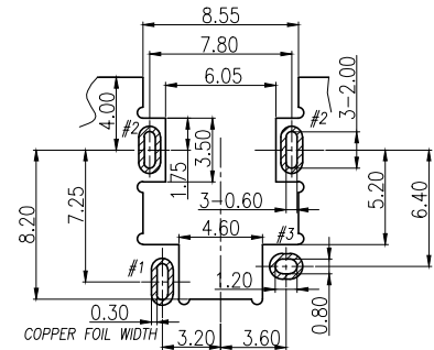
RECOMMEND P.C.B LAYOUT (TOLERANCES:±0.05) TOP VIEW
