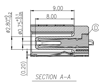
MATING PLUG TOLERANCE:X.XX:±0.10 PLUG 型號 皇積 45P06CV230-1A00-01
