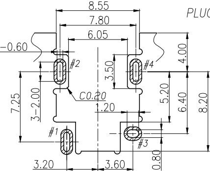
RECOMMEND P.C.B LAYOUT (TOLERANCES:±0.05) TOP VIEW
