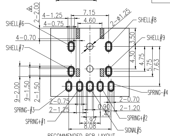
RECOMMENDED PCB LAYOUT COMPONENT SIDE (TOLERANCE: ±0.05)
