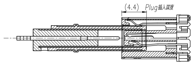
2. PIN(+) CONTACT
