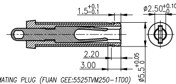
MATING PLUG (FUJAN GEE:5525VM250-1T00) TOLERANCE: X.XX:0.10
