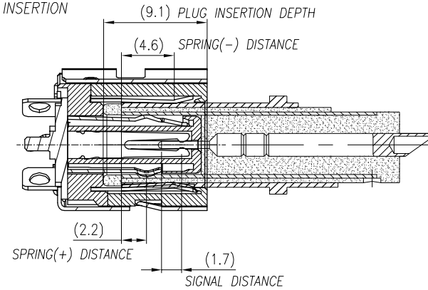
4. FULL INSERTION
