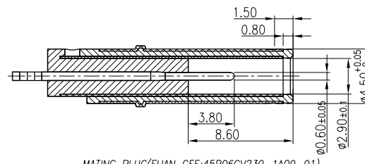
MATING PLUG(FUAN GEE:45P06CV230-1A00-01) TOLERANCE:X.XX:±0.10
