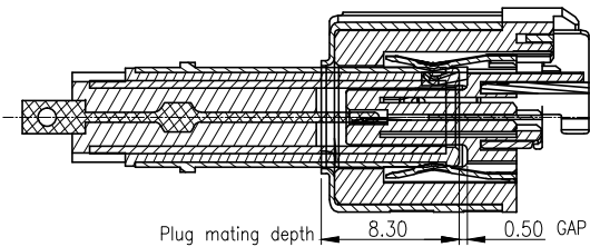
4. LOCKED STATUS
