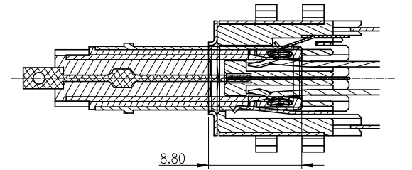
5. FULLY MATED
