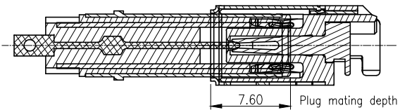
4. LOCKED STATUS
