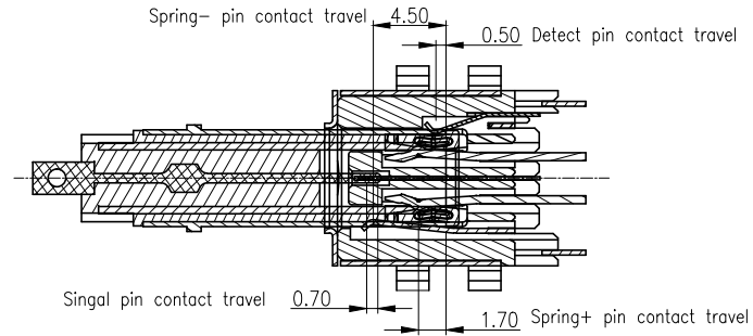
5. FULLY MATED
