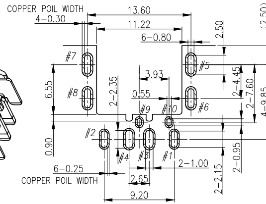
RECOMMENDED P.C.B LAYOUT TOP VIEW TOLERANCE:±0.05 THICKNESS=0.8~1.2T
