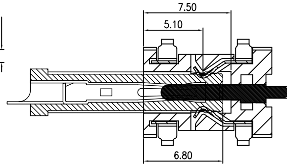
DC JACK INSERT DEPTH
