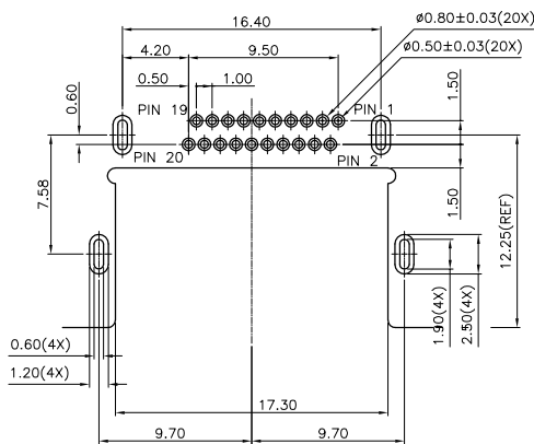
RECOMMENDED PCB LAYOUT(TOP VIEW) (THICKNESS=1.20±0.05mm) (TOLERANCE=±0.05mm)
