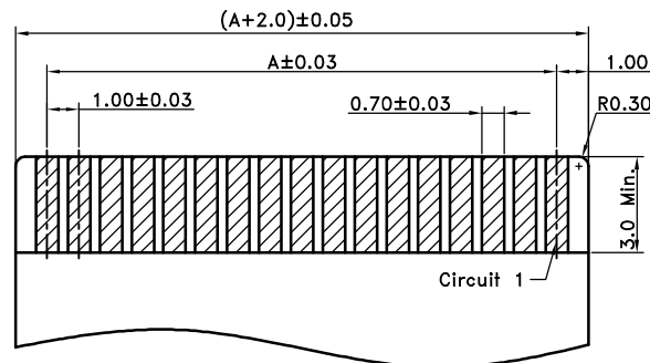
Applicable FFC Thickness 0.30mm
