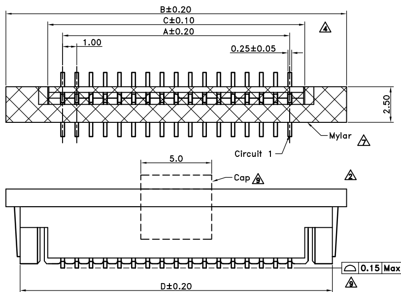
Applicable FFC Thickness 0.30mm
