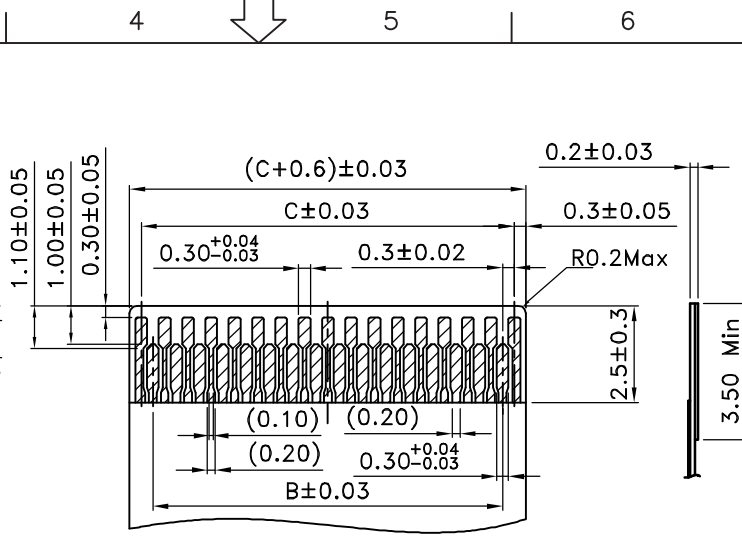
△ Recommend FPC/FFC Dimension
