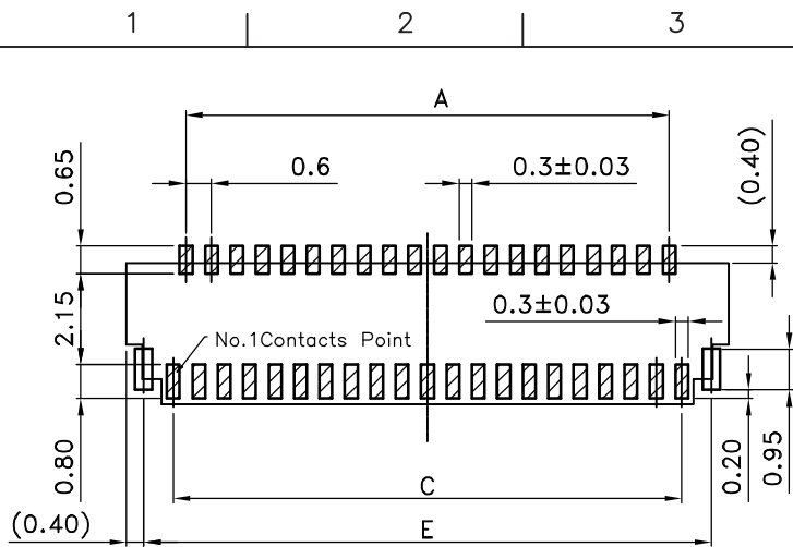
△ Recommend PCB Layout General Tolerance ±0.05
