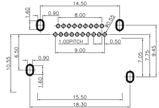
RECOMMENDED PCB LAYOUT(TOP VIEW) (THICKNESS=1.0±0.10mm) (TOLERANCE=±0.05mm)
