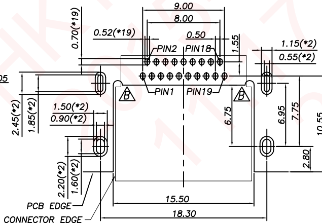
RECOMMENDED P.C.B. LAYOUT (T:1.20±0.05mm) TOLERANCE UNSPECIFIED ±0.05mm
