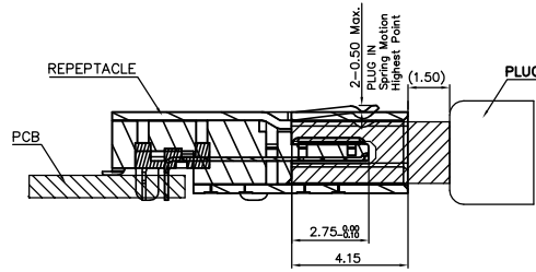
PULG INSERTION DEPTH
