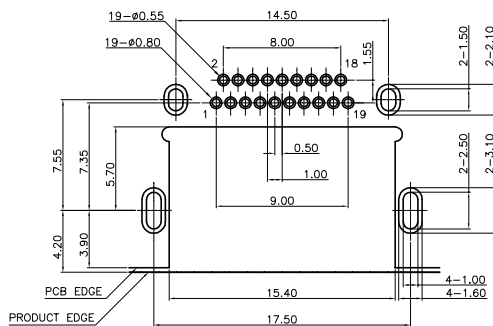
RECOMMENDED PCB LAYOUT(TOP VIEW) (THICKNESS=1.2±0.10mm) (TOLERANCE=±0.05mm)
