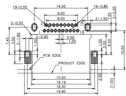
RECOMMENDED PCB LAYOUT(TOP VIEW) (DEFAULT DIMENSION TOL=±0.05mm) (THICKNESS=1.0±0.10mm) *STAND-OFF AREA
