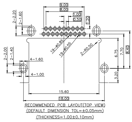
HDMI TYPE A PIN ASSIGNMENT
