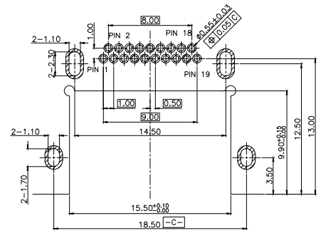
RECOMMENDED PCB LAYOUT(TOP VIEW) (THICKNESS=1.2±0.10mm) (TOLERANCE=±0.03mm)
