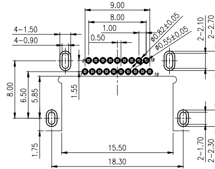
RECOMMENDED PCB LAYOUT (COMPONENT SIDE) TOP VIEW DEFAULT TOLERANCES ±0.05mm P.C.B THICKNESS=1.00mm
