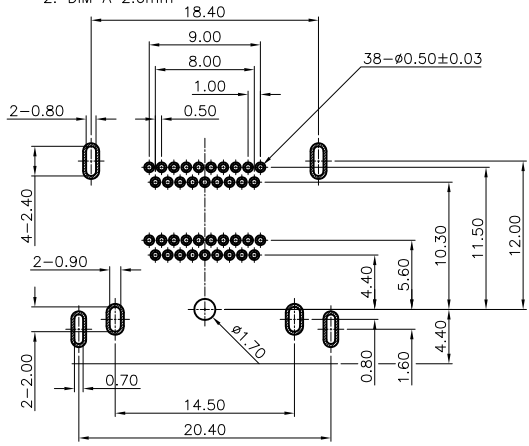
RECOMMENDED PCB LAYOUT(TOP VIEW) (THICKNESS=1.6±0.10mm) (TOLERANCE=±0.05mm)
