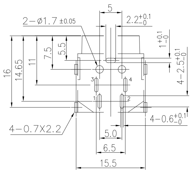
PCB LAYOUT (SOLDER SIDE) TOLERANCE: ±0.05
