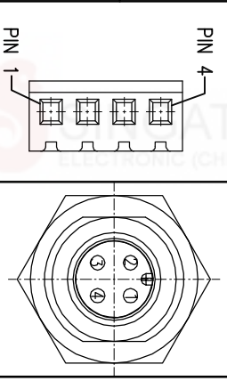
Pin Assignments Front View
