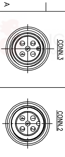
PIN ASSIGNMENTS
