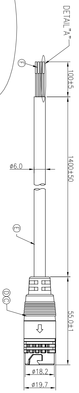
CONN.1 WATERPROOF RATE: IP67
