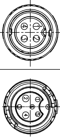
Pin Assignments Front View
