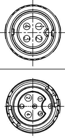
Pin Assignments Front View
