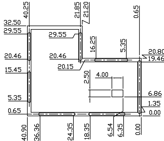
PCB LAYOUT
