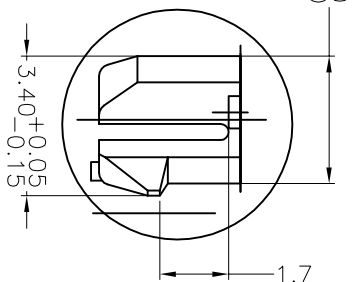
VIEW A SCALE 3:1
