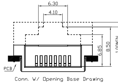
Conn. W/ Opening Base Drawing
