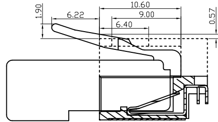
Conn. W/ Opening Base W/Plug Section Drawing
