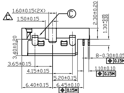
Conn. W/ Opening Base Drawing
