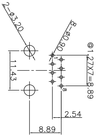
PC Board Layout Component Side Shown
