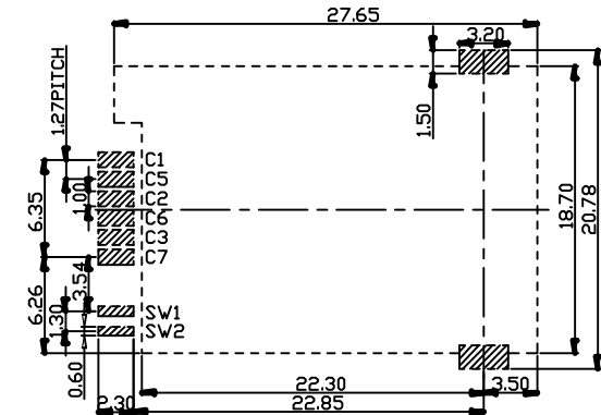
The recommended pcb layout (Tolerance=±0.05mm)
