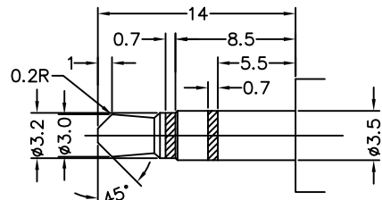
MEETING PLUG SINGATRON P/N:2SP-353P-001
