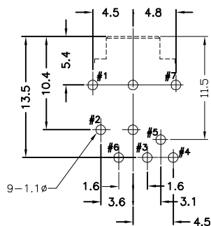
RECOMMENDED P.C.B LAYOUT TOP VIEW (TOLERANCE: ±0.05)
