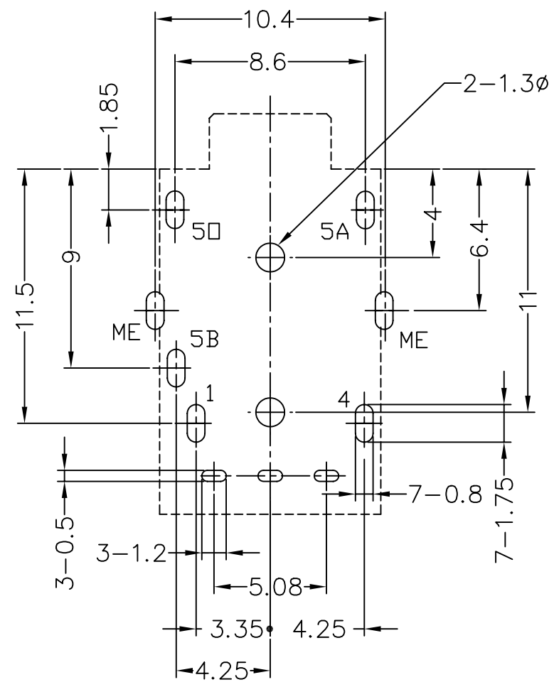
RECOMMENDED PCB LAYOUT COMPONENT SIDE (TOLERANCE: ±0.05)
