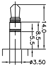
RECOMMENDED PLUG 3-POLE
