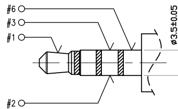
φ3.5-(4)POLE PLUG
