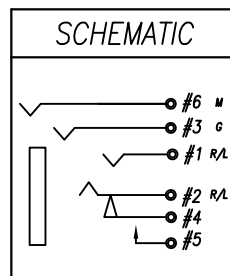
φ3.5-(4)POLE PLUG
