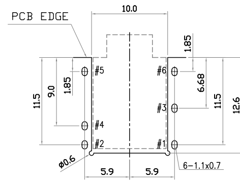
Recommend of PC Board Holes Tolerance : ±0.05(Printed-Top view)
