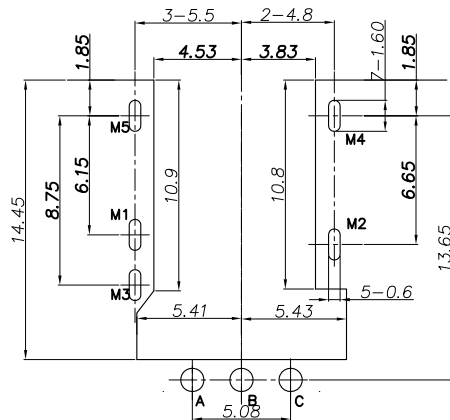
RECOMMENDED P.C.B LAYOUT BOTTOM VIEW(TOL.±0.05)
