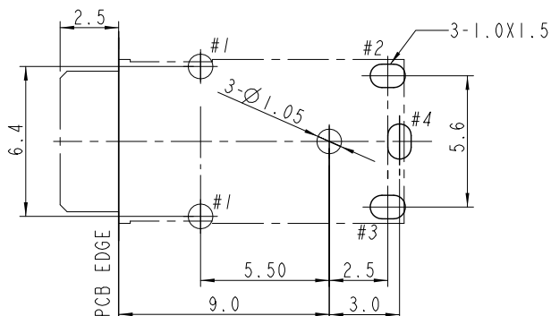
RECOMMENDED PCB LAYOUT TOP VIEW (TOL ±0.05, THK 1.6±0.05)
