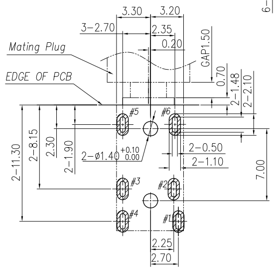
RECOMMENDED PCB LAYOUT T=1.20 TOP VIEW (TOLERANCE: ±0.05)
