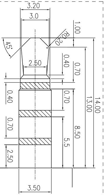
3.5Ø 4POLE PLUG (TOLERANCE:±0.05)
