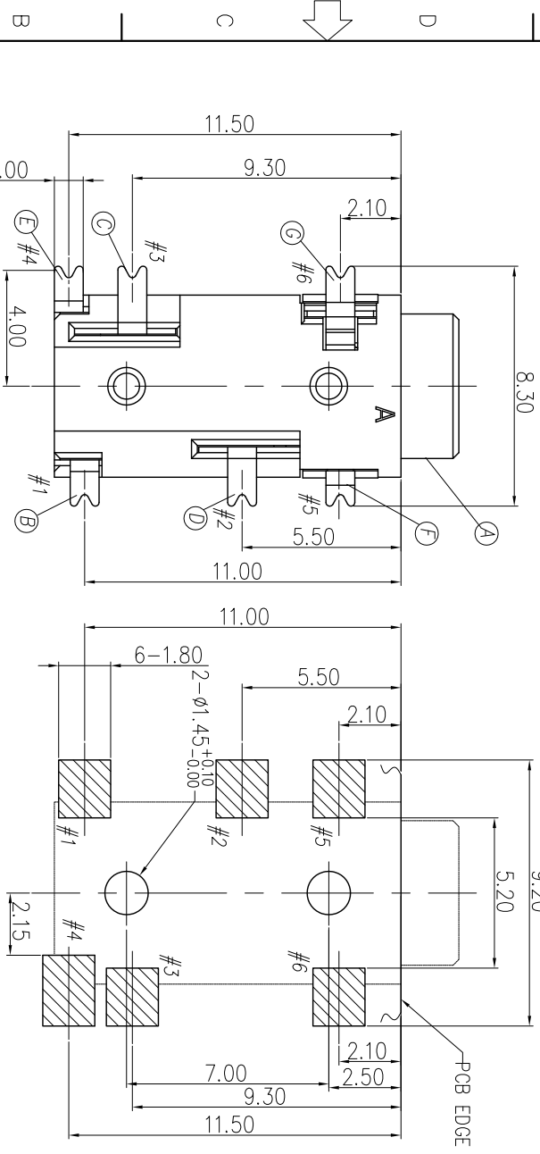
RECOMMENDED PCB LAYOUT TOP VIEW (TOLERANCE: ±0.05)
