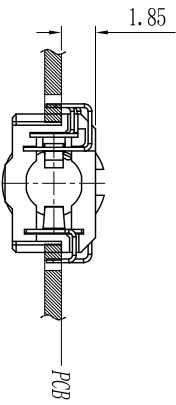
RECOMMENDED P.C.B. LAYOUT TOP VIEW (TOLERANCE: ±0.05)
