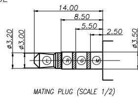
MATING PLUG (SCALE 1/2)
