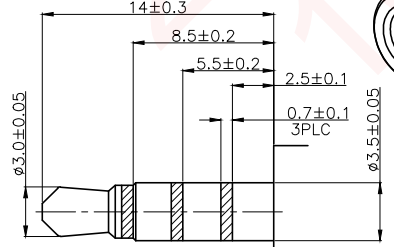
RECOMMENDED PLUG 4-POLE(TOLERANCE: ±0.05)
