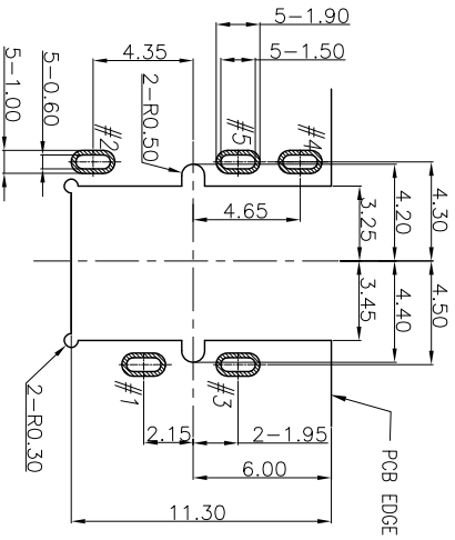
RECOMMENDED PCB LAYOUT(TOP VIEW) (TOLERANCE: ±0.05)
