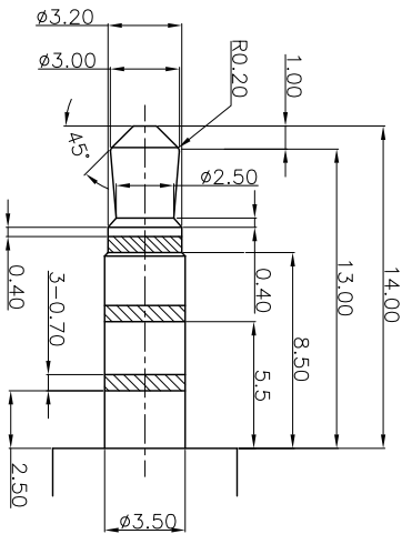
3.50 4POLE PLUG(TOLERANCE: ±0.05)
