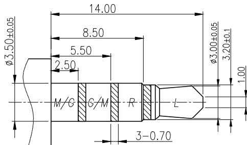
RECOMMENDED PLUG;TOL.±0.05 Ø3.5 4-POLE STANDARD PLUG
