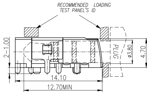
RECOMMENDED PLUG;TOL.±0.05 Ø3.5 4-POLE STANDARD PLUG
